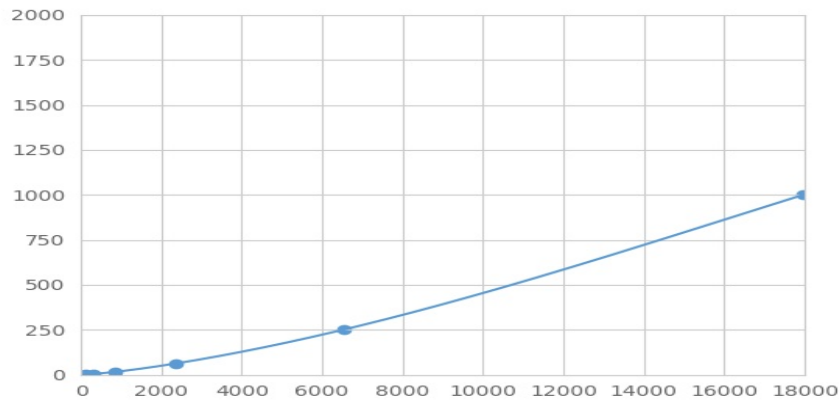
Typical Standard Curve for TNFSF14 Magnetic Luminex Assay.
