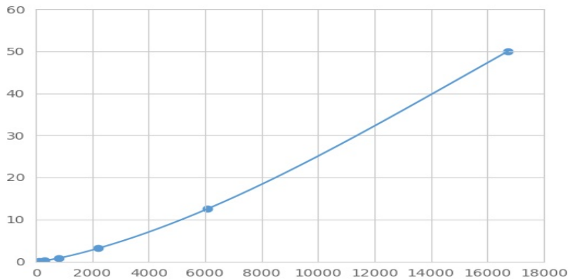
Typical Standard Curve for UQCR Magnetic Luminex Assay.
