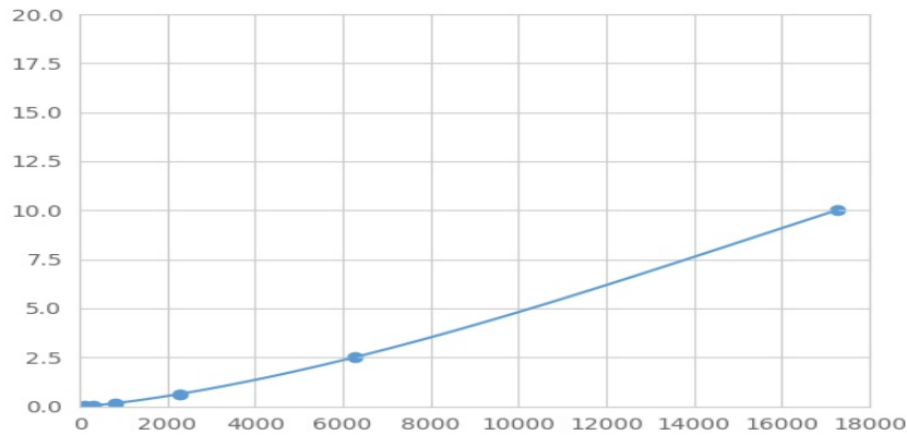
Typical Standard Curve for VIPR1 Magnetic Luminex Assay.
