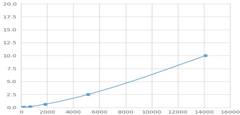
Typical Standard Curve for WT1 Magnetic Luminex Assay.
