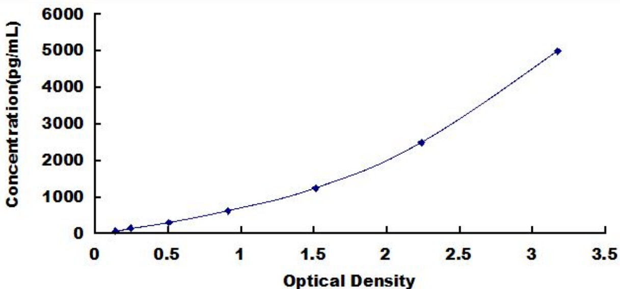
Typical Standard Curve for CC16, Mouse ELISA.
