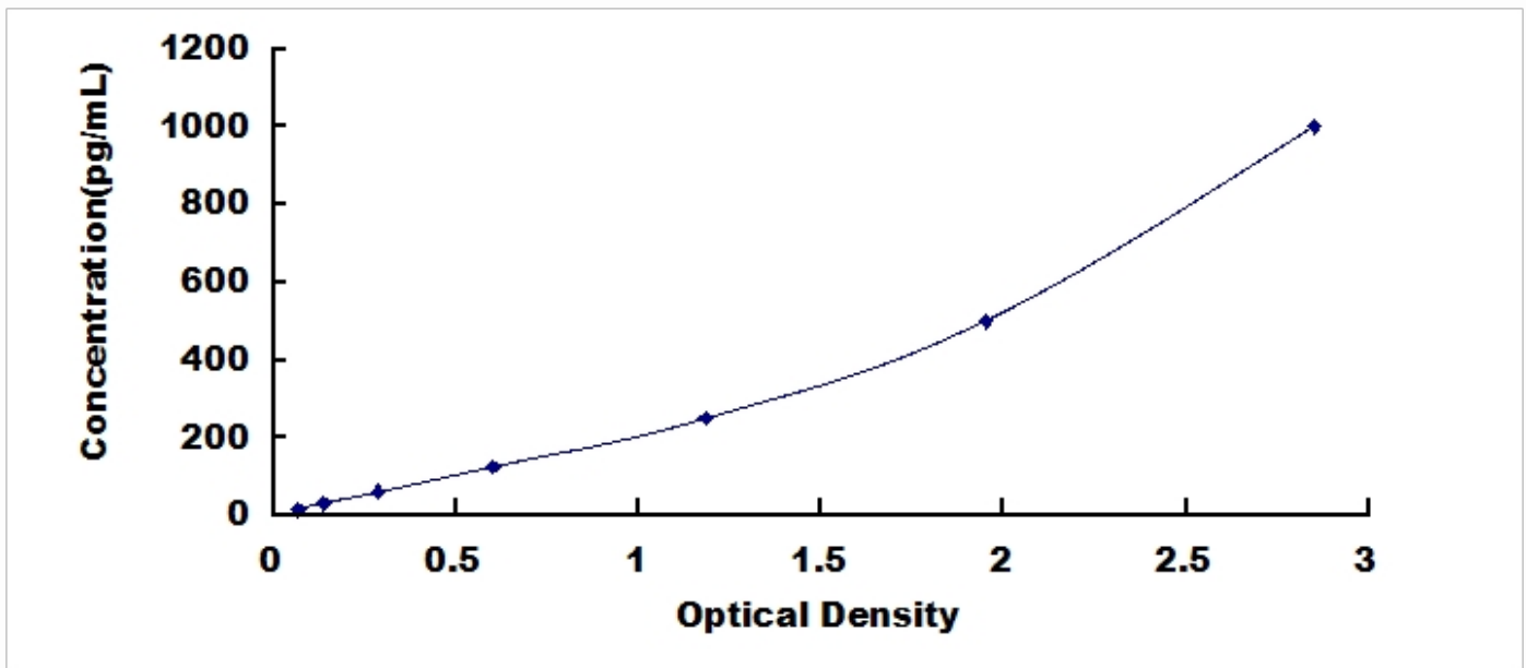
Typical Standard Curve for SCF, Mouse ELISA.
