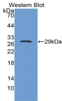
Figure. Western Blot; Sample: Recombinant IGFBP5, Rat.
