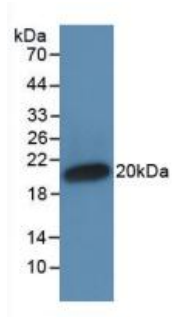
Figure. Western Blot; Sample: Recombinant IFNa, Human.
