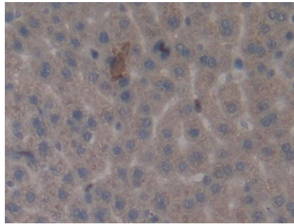
DAB staining on IHC-P; Samples: Rat Liver Tissue.
