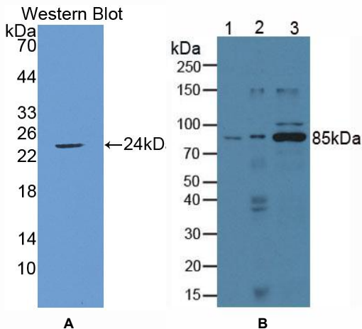
Figure 1. Western Blot
