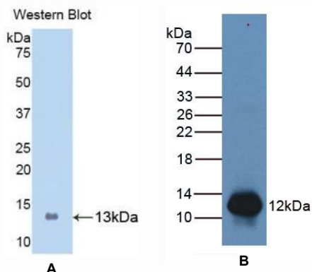
Figure 1. Western Blot
