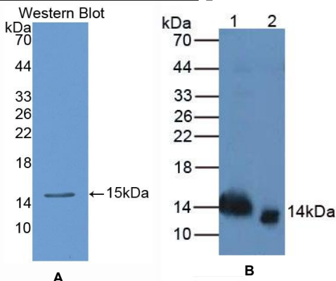
Figure 1. Western Blot
