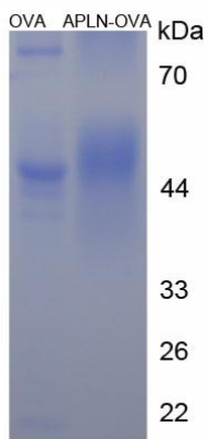
Figure 1. SDS-PAGE of OVA Conjugated APLN
