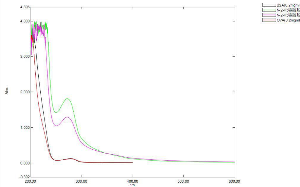
Figure 1. UV-spectrum
