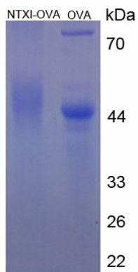
Figure 3. SDS-PAGE of OVA Conjugated NTXI
