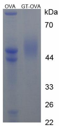
Figure 1. SDS-PAGE of OVA Conjugated GT
