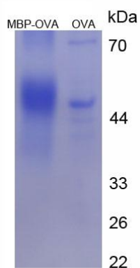
Figure 2. SDS-PAGE of OVA Conjugated MBP
