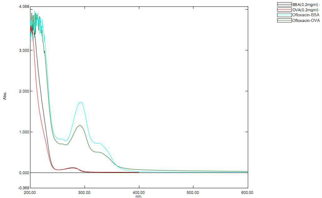
Figure 1. UV-spectrum
