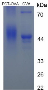
Figure 2. MASS Spectrometry of the Original Peptide
