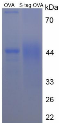
Figure 1. SDS-PAGE of OVA Conjugated S-tag
