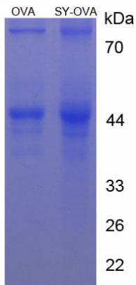
Figure 1. SDS-PAGE
