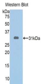
Figure. Western Blot; Sample: Recombinant ABCA1, Human.
