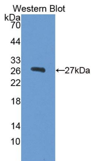
Figure. Western Blot; Sample: Recombinant AFP, Human.
