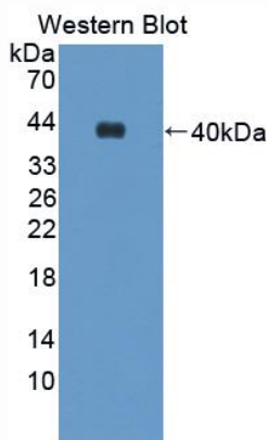
Used in Western Blot, Sample: Recombinant ALAD, Rat
