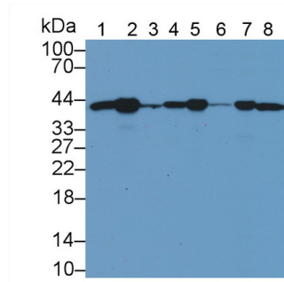
Western Blot; Sample: Lane1: Rat Cerebrum lysate; Lane2: Rat Heart lysate; Lane3: Mouse Liver lysate; Lane4: Mouse Cerebrum lysate; Lane5: Mouse Heart lysate; Lane6: Porcine Liver lysate; Lane7: Porcine Cerebrum lysate; Lane8: Porcine Heart lysate Primary Ab: 1µg/mL Rabbit Anti-Multi-species ACTb Ab Second Ab: 0.2µg/mL HRP-Linked Caprine Anti-Rabbit IgG Polyclonal Antibody (Catalog: SAA544Rb19)
