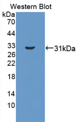
Used in Western Blot, Sample: Recombinant CTBP1, Human
