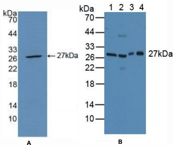
Figure 1. Western Blot
