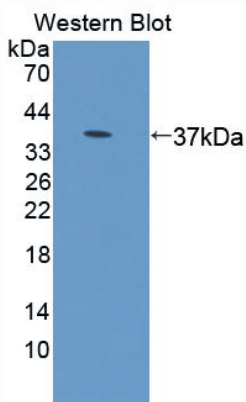
Used in Western Blot, Sample: Recombinant CBR1, Rat
