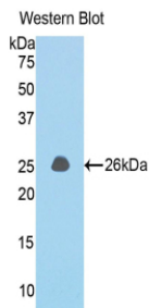
Figure. Western Blot; Sample: Recombinant CCDC80, Rat.
