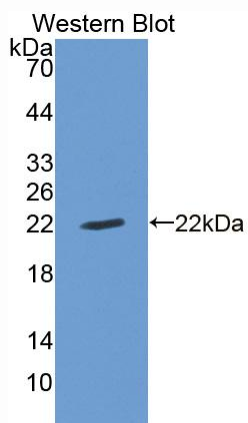
Used in Western Blot, Sample: Recombinant CDKN1A, Rat
