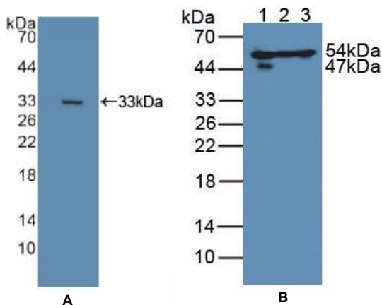
Figure 1. Western Blot
