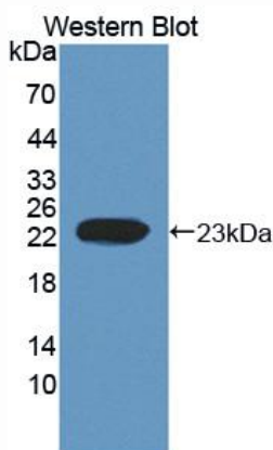
Used in Western Blot, Sample: Recombinant EFNA1, Human
