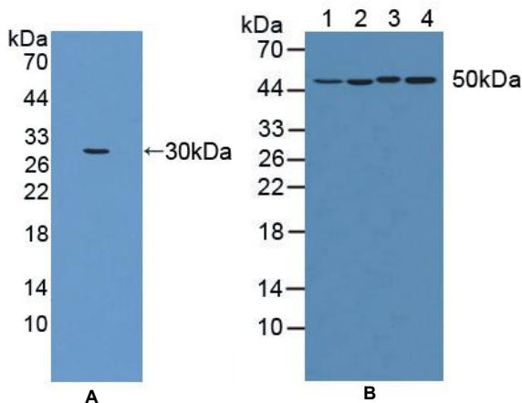
Figure 1. Western Blot
