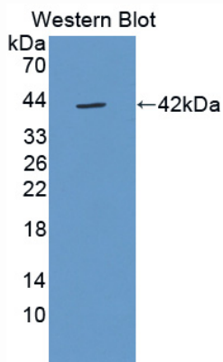
Used in Western Blot, Sample: Recombinant FKBPL, Human
