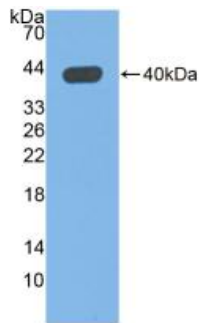
Figure. Western Blot; Sample: Recombinant QPCT, Human.
