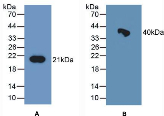
Figure 1. Western Blot
