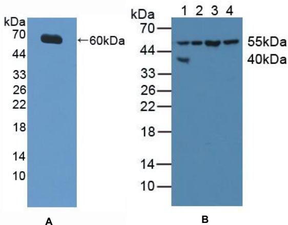
Figure 1. Western Blot
