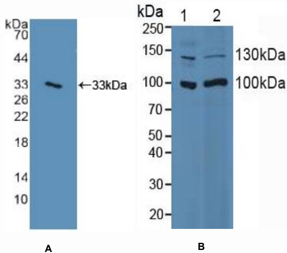
Figure 1. Western Blot
