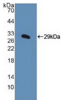
Figure. Western Blot; Sample: Recombinant KPNa1, Human.
