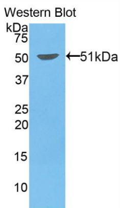
Used in Western Blot, Sample: Recombinant KIF5A, Mouse
