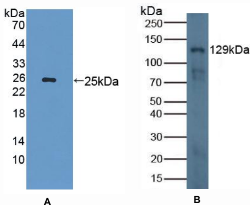
Figure 1. Western Blot
