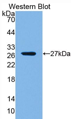
Used in Western Blot, Sample: Recombinant LOXL1, Mouse
