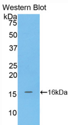
Used in Western Blot, Sample: Recombinant MGP, Rat
