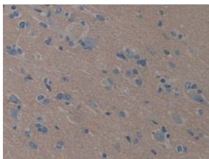
Figure. DAB staining on IHC-P; Samples: Human Brain Tissue.
