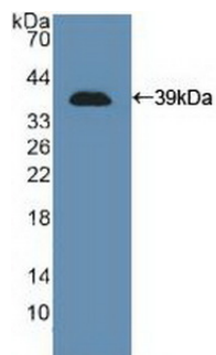
Figure. Western Blot; Sample: Recombinant NCAM, Human.
