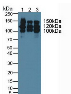
Figure. Western Blot; Lane1: Porcine Brain Tissue; Lane2: Mouse Brain Tissue; Lane3: Rat Brain Tissue.
