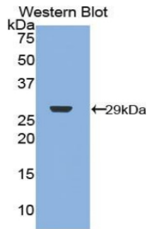
Figure. Western Blot; Sample: Recombinant NF2, Human.
