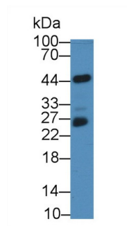
Western Blot; Sample: Mouse Serum; Primary Ab: 2 \mu g/mL Rabbit Anti-Human NF2 Antibody Second Ab: 0.2 \mu g/mL HRP-Linked Caprine Anti-Rabbit IgG Polyclonal Antibody (Catalog: SAA544Rb19)
