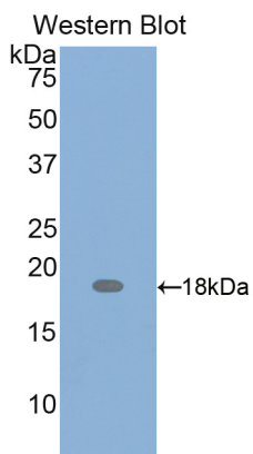
Used in Western Blot, Sample: Recombinant PTHrP, Mouse
