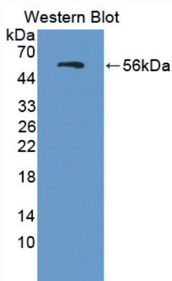
Used in Western Blot, Sample: Recombinant FARS2, Rat
