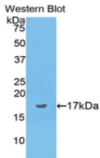
Figure. Western Blot; Sample: Recombinant VP, Rat.
