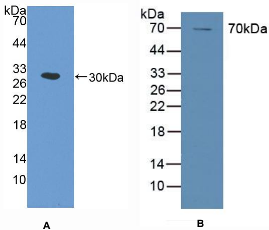
Figure 1. Western Blot
