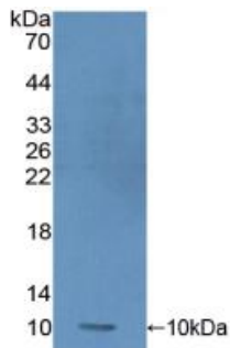
Figure. Western Blot; Sample: Recombinant PRM1, Human.
